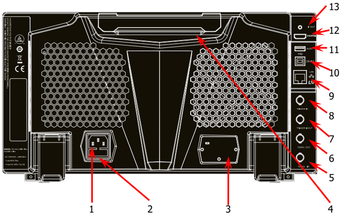
Figure 2 Rear Panel
