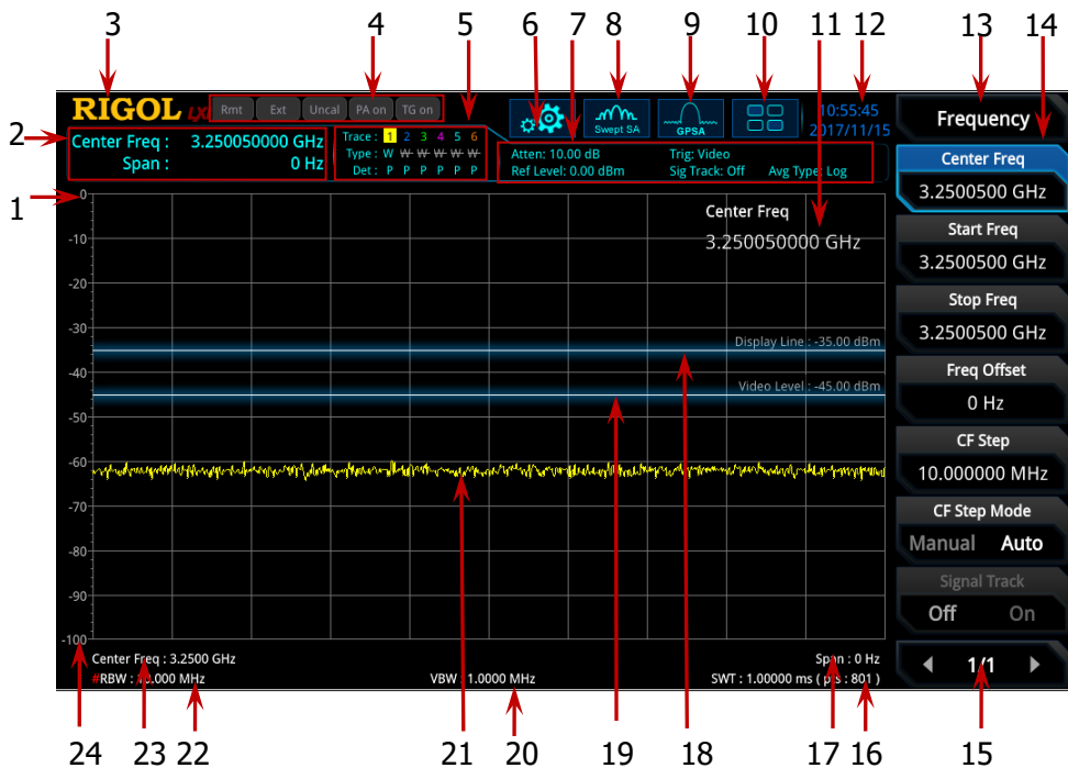
Figure 1-9 User Interface
