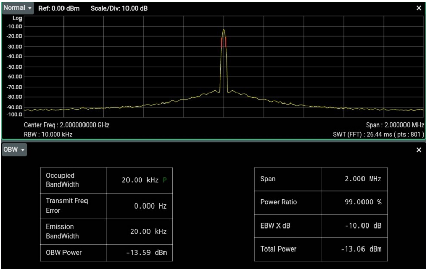
Figure 5.8 OBW Measurement Interface
