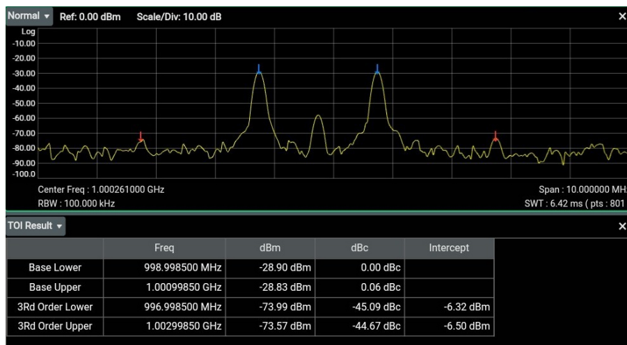
Figure 5.6 TOI Distortion Measurement Interface
